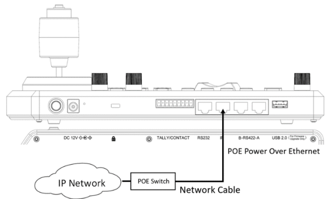
Power using POE
