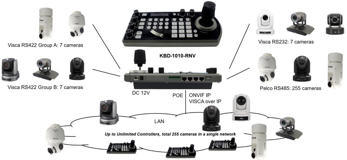
Cross Protocol Mix-control with RS232/RS422 and IP in one single system
