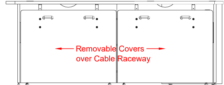
REAR VIEW
