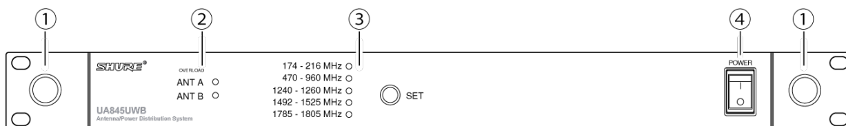
Front Panel
