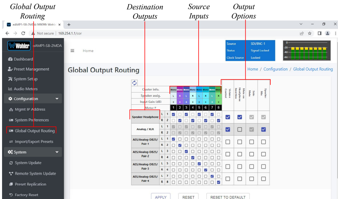
Figure 4-18: Global Output Routing
